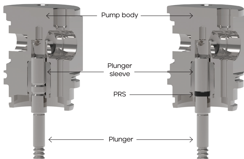
Plunger ring seal design
