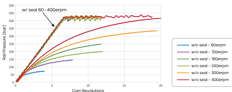
Rail pressure build at low RPM: Standard vs PRS pump
